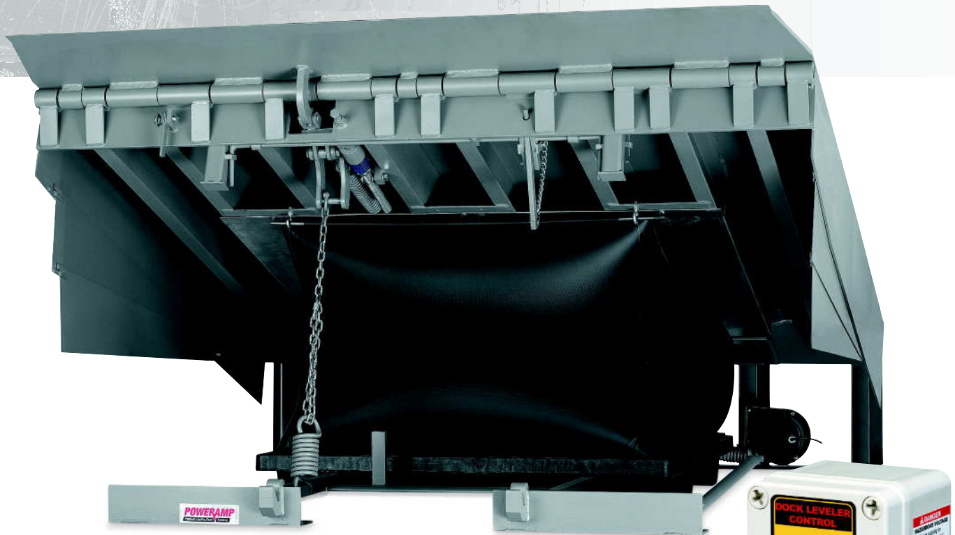
AP Series 7'x 8' 35,000 CIR with CleanSweep Frame™ shown.
